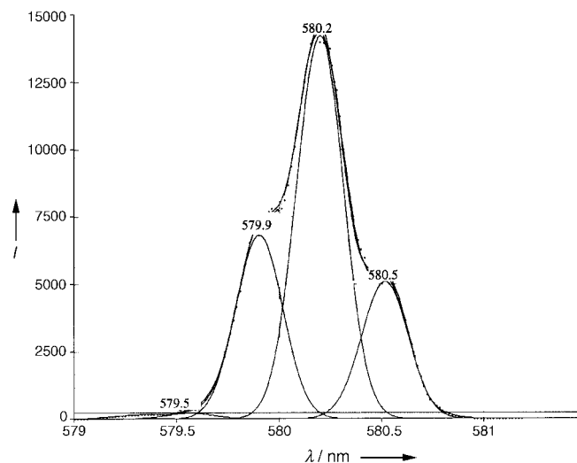
Figure 4. Laser excitation spectrum of the \text{Eu}^{3+} compound showing the overlapping excitation bands of the four different \text{Eu}^{3+} sites. The \text{Eu}^{3+} emission due to the ^5\text{D}_0 to ^7\text{F}_2 transition was monitored.
